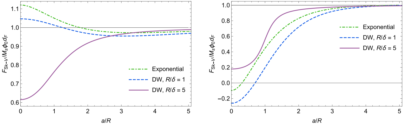
FIG. 3. The dependence of the normalized interaction free energy, \mathcal{F}_{\text{Sk-v}} , on a/R for the chirality \eta = +1 (left) and \eta = -1 (right). The ratio of the skyrmion radius and the Pearl length is unity, \lambda/R = 1 (see text).
