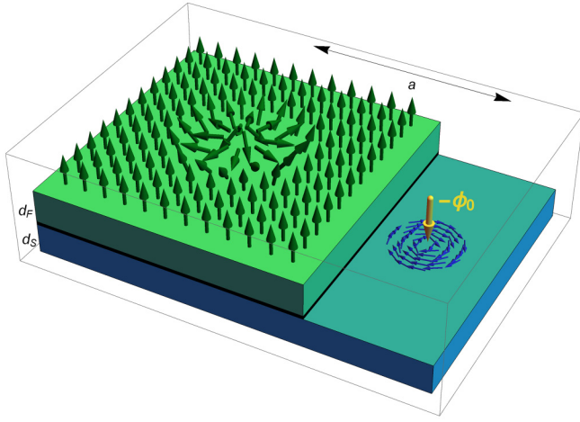
FIG. 1. Sketch of a ferromagnet (green) - superconductor (blue) heterostructure. There is also a thin insulating layer (black) which suppresses the proximity effect. The ferromagnetic layer hosts a Néel-type skyrmion. The magnetic profile of the skyrmion with the positive chirality is schematically shown. The superconducting layer hosts a vortex at some distance from the skyrmion's center. The vortex is shown schematically by blue lines, the yellow arrow points towards the direction of its magnetic flux. d_F and d_S denote the width of the ferromagnet and superconductor film, respectively (see text).
