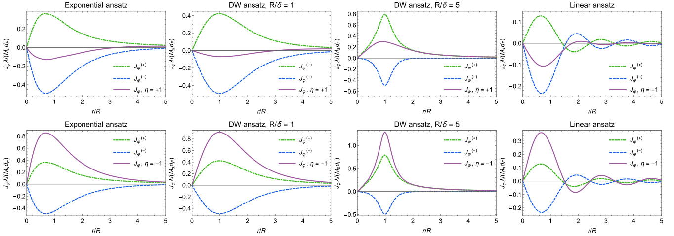
FIG. 2. The dependence of J_\varphi^{(\pm)} and the total supercurrent J_\varphi on the distance from the skyrmion center for the cases of positive (top) and negative (bottom) chiralities. The parameters are d_S/\lambda_L = 0.01 , d_F/\lambda_L = 0.005 , and R/\lambda_L = 3 . The supercurrent is calculated for the exponential, domain wall (DW) and linear ansatz.
