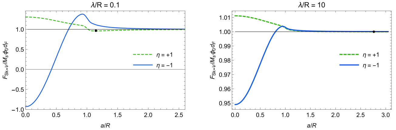
FIG. 4. The dependence of the normalized interacting free energy, \mathcal{F}_{\text{Sk-v}} , on a/R for the linear ansatz for the skyrmion's profile. The plots are for two chiralities and for two values of ratio of the skyrmion radius and the Pearl length: \lambda/R = 0.1 (left) and 10 (right). Black dot near a \approx 1.2R on the left panel marks the location of the global minimum of the interaction energy. For \lambda/R = 10 (right), the global minimum is resided at a \approx 2.8R (see text).
